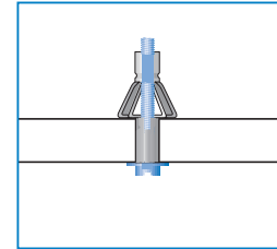
Molly screw anchor (comparable with Hilti HHD)
